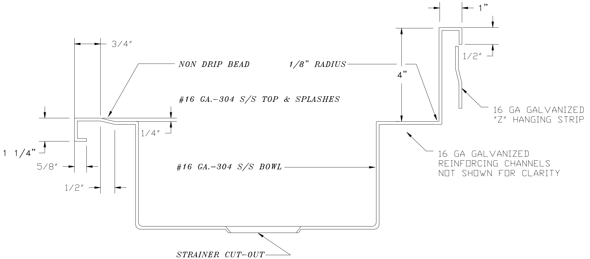
TYPICAL S/S SINKTOP
