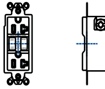
Duplex Outlet, G.F.I. 20A, 125V Commercial Grade Grey
