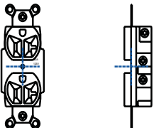
Duplex Outlet 20A, 125V Specification Grade Grey
