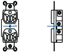
Duplex Outlet 20A, 125V Specification Grade Grey
