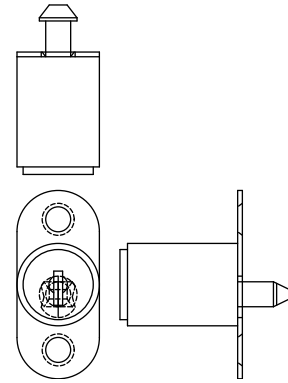
Five-Disk Tumbler Sliding Door Lock
