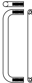
Satin Chrome Plated Sq. Bar Pull, 4" Centers
