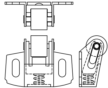
Nylon Tired Roller Catch
