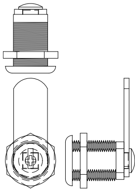
Five-Disk Tumbler Door & Drawer Cam Lock
